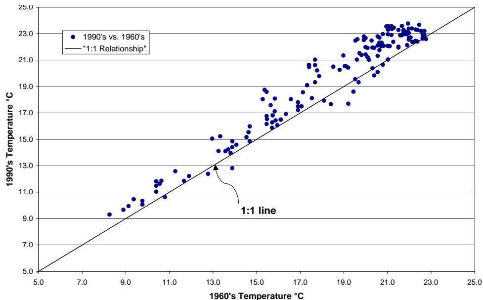
Figure 4.5 Comparison of Decadal Average Daily Maximum Water Temperature for the NRW at Stillwater Dam in Cherryfield, ME (1960s vs 1990s).
